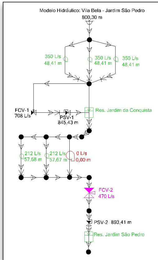
The hydraulic model of the water network in WaterCAD.
